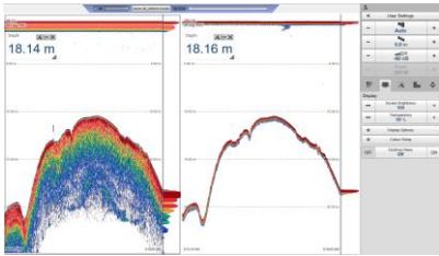
EA440 echogram view at 38 kHz and 200 kHz
