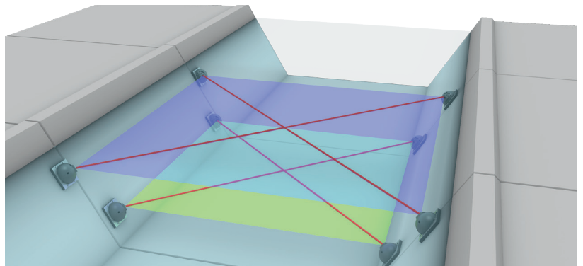
Multi-path Kanalıs system with crossed paths in two planes
