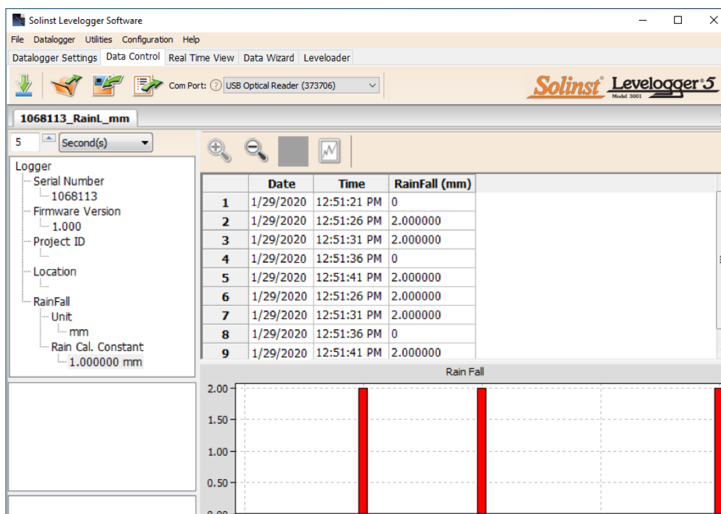
Figure 7-2 Rainlogger Data
