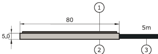
Figure 3 dimensions in mm: heater (1) heat flux sensor body (2), cable (3)
